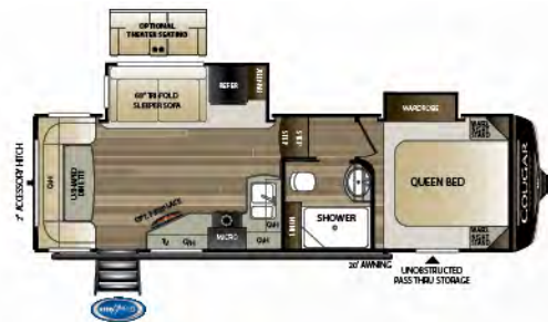
24RDS | Rear dinette, two slides Weight: 7300 LBS. | Length: 28'6"
