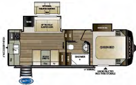
23MLS | Short, rear kitchen w/ wardrobe slide Weight: 7140 LBS. | Length: 26'10"
