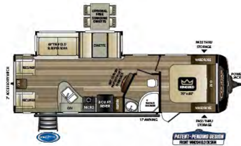
27SAB | Rear living room, side-aisle bath Weight: 6679 LBS. | Length: 31' 5"
