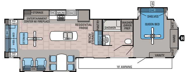
JAY FLIGHT BUNGLOW | 40RLTS OPTIONS: C, D
