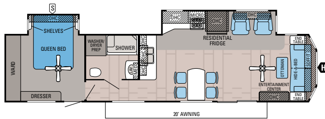
JAY FLIGHT BUNGLOW | 40FSDS OPTIONS: C, D
