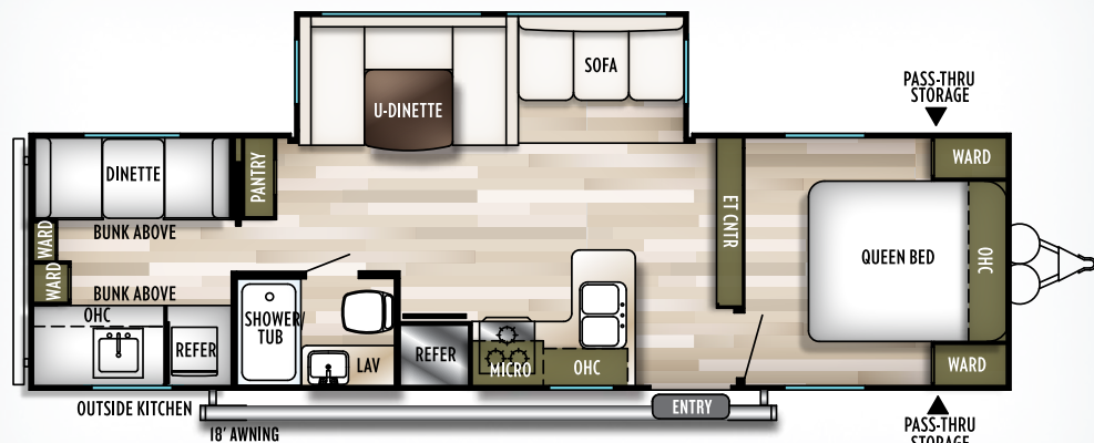
30KQBSS | DRY WEIGHT 6,780
