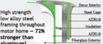
High strength low alloy steel framing throughout motor home - 72% stronger than aluminum! No wood in side walls or roof!
