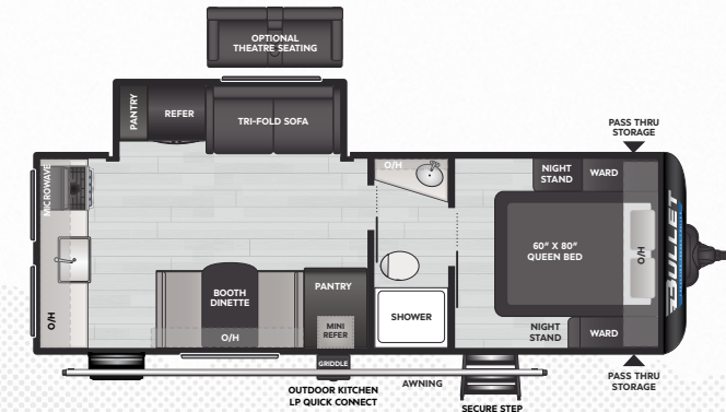
245RKS | WEIGHT TBD | LENGTH 28' 8"
