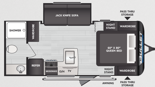
1840RB | WEIGHT 4337 | LENGTH 22' 11"
