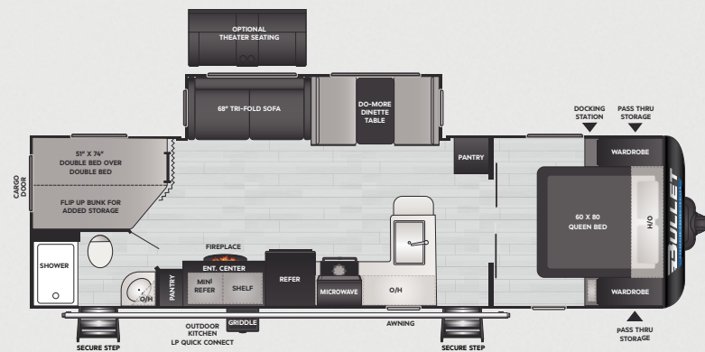
290BHS | WEIGHT 6525 | LENGTH 33' 3"
