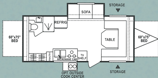
23CMS-UVW 4000 • Length 24'6"
