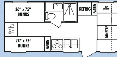
CS210-UVW 2966 • Length 22'9"
