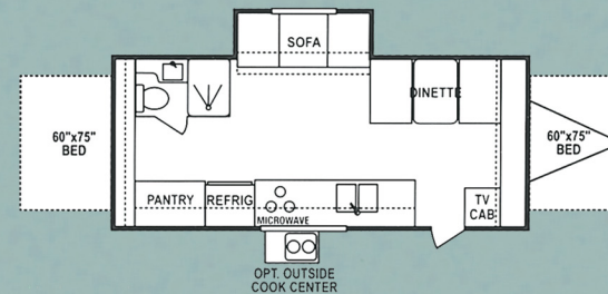
23CS-UVW 4151 • Length 24'6"
