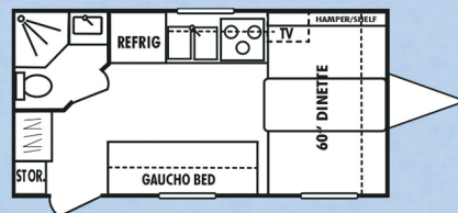
CS162-UVW 2370 • Length 19'1"
