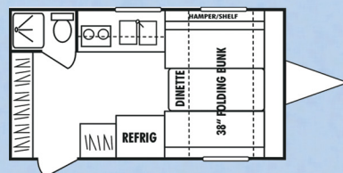
CS130-UVW 2073 • Length 16'11"
