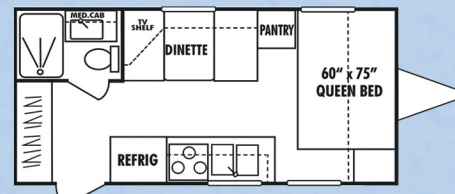
CS180-UVW 2962 • Length 21'9"
