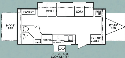
22CP-UVW 4170 • Length 23'4"
