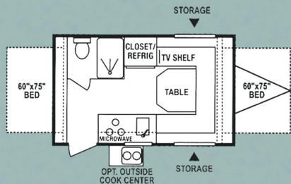
16C-UVW 2654 • Length 17'7"
