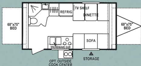
20C-UVW 3205 • Length 20'5"
