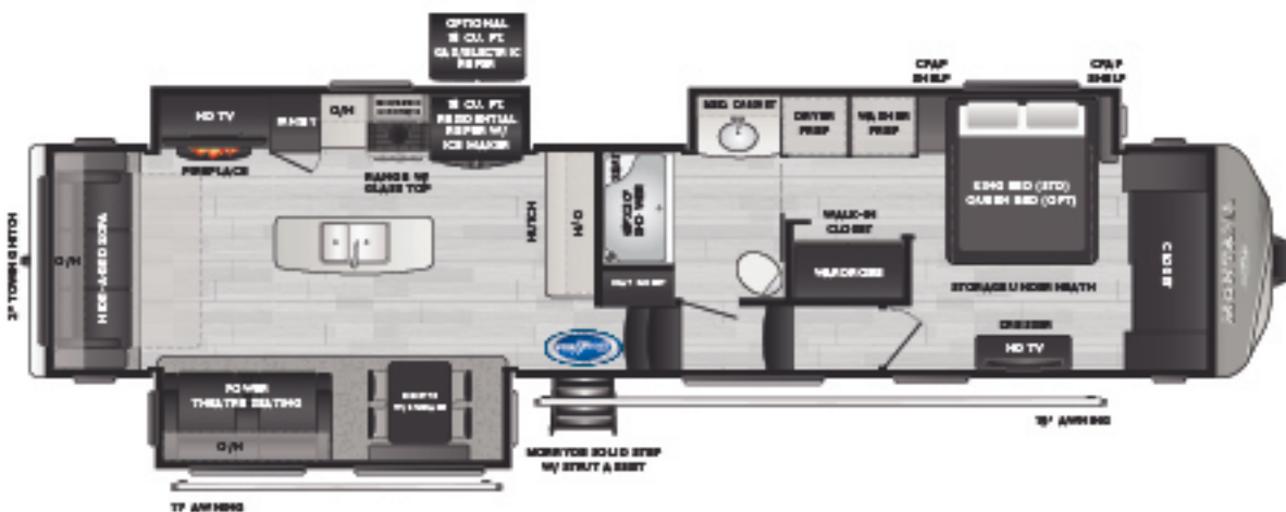
3813MS Rear living room w/ master suite & walk-in closet WEIGHT 13763 LENGTH 40' 9"
