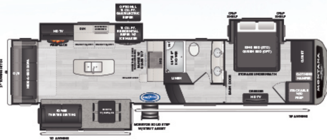
3231CK Center kitchen, three slides, dual vanity WEIGHT 12752 LENGTH 37' 5"
