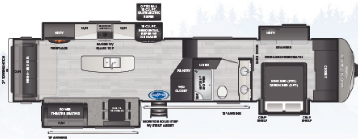
3781RL Rear living w/ double vanity bathroom & double slide bedroom WEIGHT 13485 LENGTH 41' 0"
