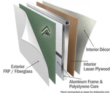
RV Sidewall Cut-Away (Exploded View)
