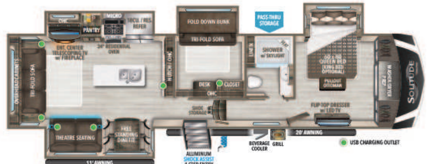
378MBS UVW' HITCH' GVWR LENGTH' HEIGHT CAPACITY 378MBS-R 14,344 2,686 16,800 40' 2" 13' 5" 81 106 53
