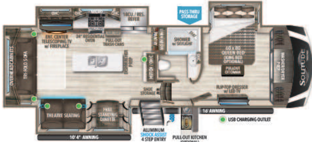
310GK UVW' HITCH' GVWR LENGTH' HEIGHT CAPACITY 310GK-R 12,100 2,350 15,000 34' 11" 13' 5" 81 106 53
