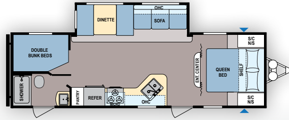
Lantern | 263BH
