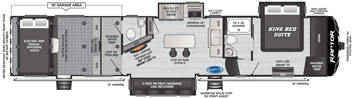
415 | WEIGHT 16065 | LENGTH 44' 0"
