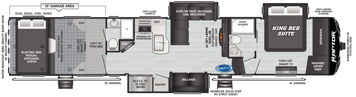
431 | WEIGHT 16316 | LENGTH 44' 11"
