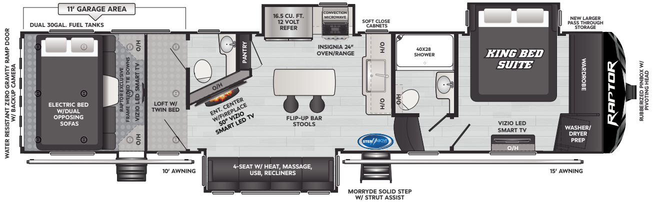
352 | WEIGHT 14705 | LENGTH 39' 0"
