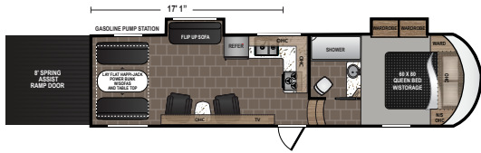
ENDURANCE | 3006 | Sleeps 4-6 Ext. Length: 33' 6" Ext. Height: 13' 4" Weight: 10,516 lbs.
