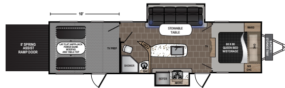
ENDURANCE | 3706 | Sleeps 4-6 Ext. Length: 36' 8" Ext. Height: 12' 4" Weight: 9,619 lbs.
