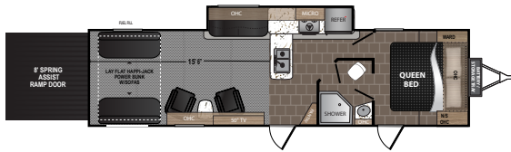
ENDURANCE | 3316 | Sleeps 4-6 Ext. Length: 36' 6" Ext. Height: 12' 4" Weight: 9,292 lbs.
