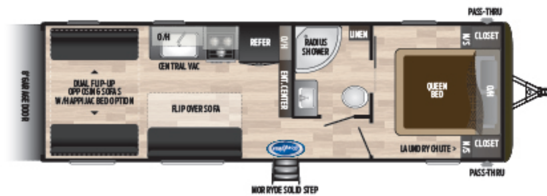
25TH | New non-slide, toy hauler w/ happijac in rear Weight: 6190 LBS. | Length: 29' 11"
