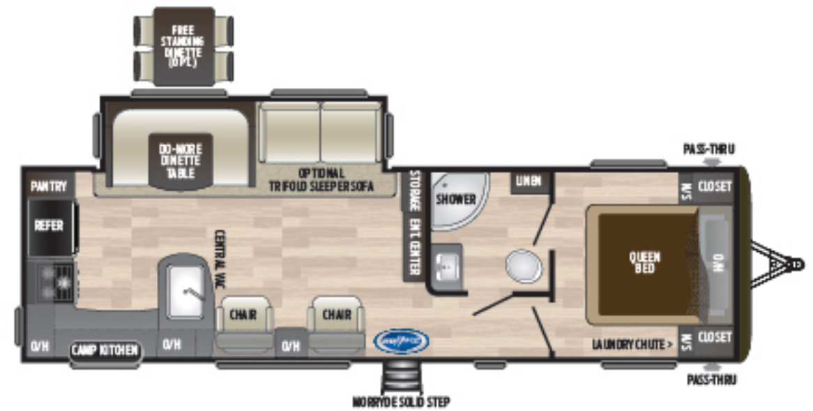
28RKS | One-slide, rear kitchen w/ recliners, camp kitchen, walk through bathroom Weight: 6969 LBS. | Length: 32' 11"
