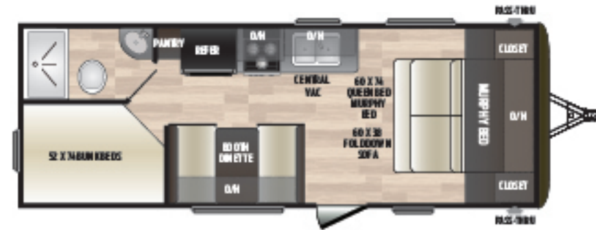
212LHS | Non-slide, double-over-double bunkhouse, murphy bed Weight: 4696 LBS. | Length: 26' 4"
