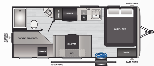
2010BH | WEIGHT 4069 | LENGTH 22' 10"
