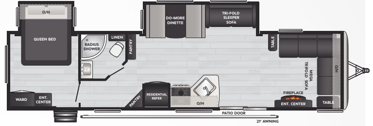
38FL | WEIGHT 8725 | LENGTH 38' 11"
