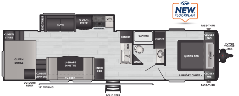
320TQ | WEIGHT TBD | LENGTH TBD
