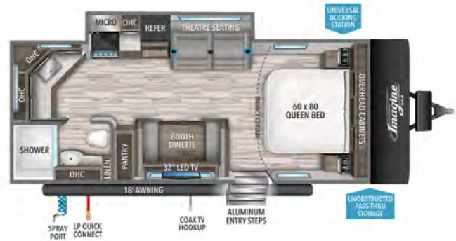
22MLE UVW' 5,176 HITCH' 490 LENGTH' 26' 11" HEIGHT 10' 5" CAPACITY 43 45 37
