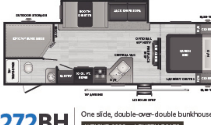
272BH | One slide, double-over-double bunkhouse, dual entry WEIGHT 6088 LENGTH 30' 7"
