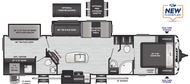
330BKQ | WEIGHT 8225 | LENGTH 37' 11"
