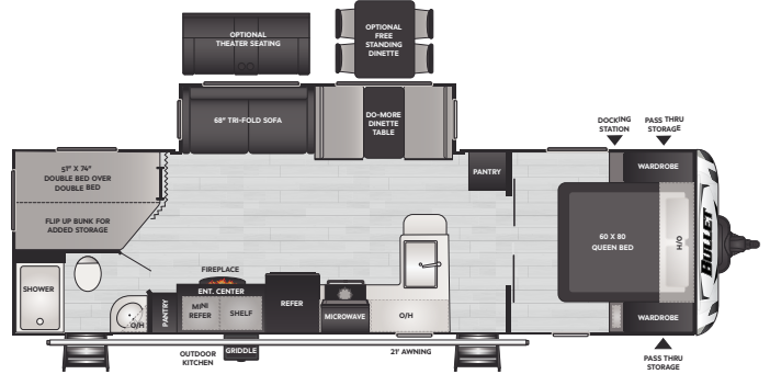
290BHS/WE | WEIGHT 6365 | LENGTH 33' 3"
