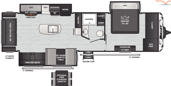
310RES | WEIGHT 7925 | LENGTH 35' 11"
