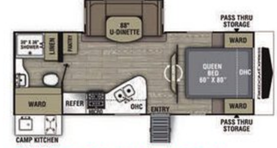
231 RBDS / Exterior Length 26' 10"
