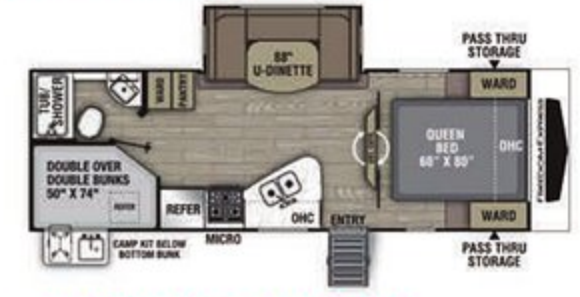
257 BHS / Exterior Length 28' 7"
