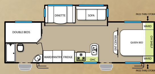
T262BHXL
