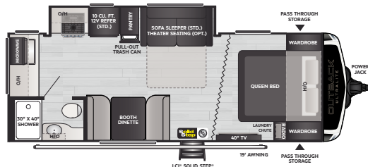
221UMD | WEIGHT 5304 | LENGTH 27' 0"
