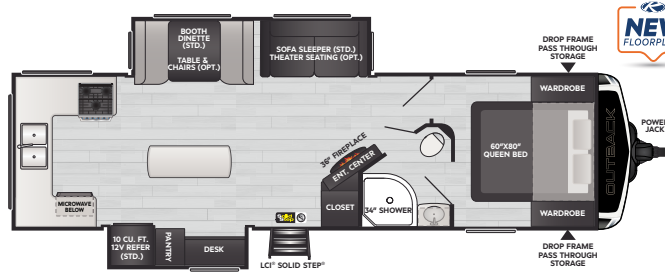
296URK | WEIGHT 7075 | LENGTH 33' 11"
