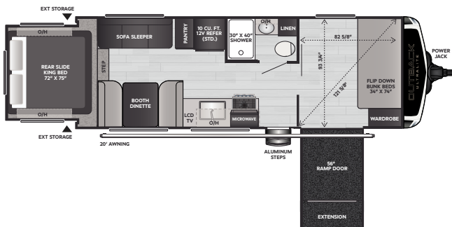
240URS | WEIGHT 5599 | LENGTH 28' 6"
