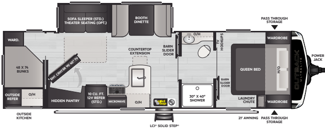
291UBH | WEIGHT 7030 | LENGTH 33' 8"
