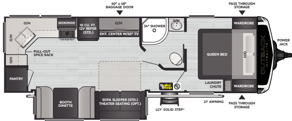
260UML | WEIGHT 6370 | LENGTH 30' 8"
