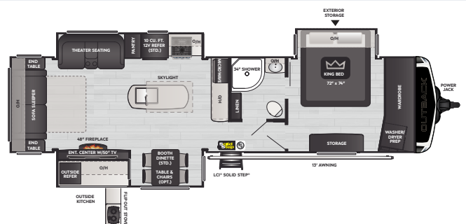
330RL | WEIGHT 8854 | LENGTH 37' 7"
