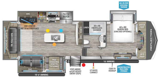
337RLS U 1 V 1 W 1 10,838 HITCH 1 2,185 LENGTH 2 35' 7" HEIGHT 3 12' 6" CAPACITY 74 87 47
