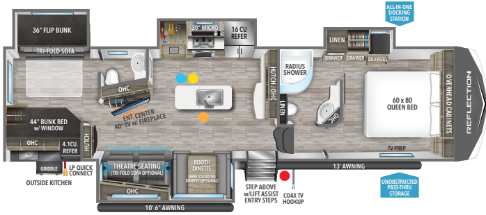
311BHS U 1 V 1 W 1 11,377 HITCH 1 2,316 LENGTH 2 36' 11" HEIGHT 3 12' 3" CAPACITY 74 87 87
