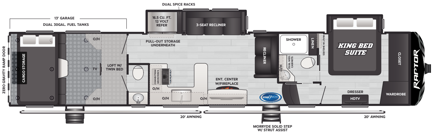
424 | WEIGHT 15605 | LENGTH 44' 6"
