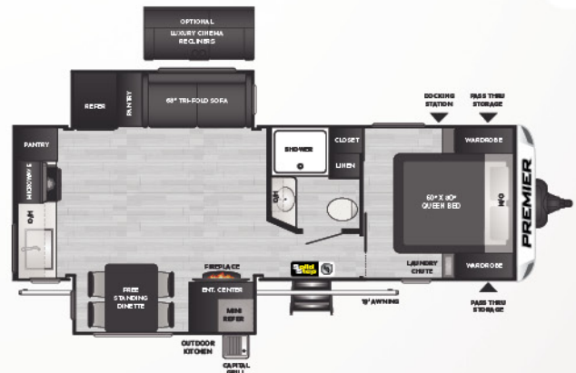
25RKPR | WEIGHT 6165 | LENGTH 29' 11" PREMIER • REAR KITCHEN, OPPOSING SLIDES
