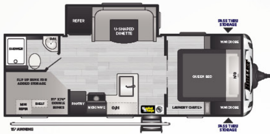
NEW! 2290BH | WEIGHT TBD | LENGTH 27' 0" CROSSFIRE • REAR BATH, DOUBLE BUNKS
