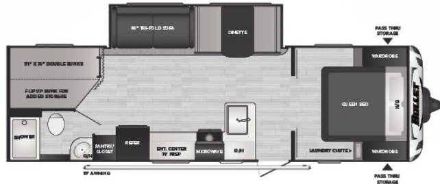
2730BHS | WEIGHT 5544 | LENGTH 31' 2" CROSSFIRE • DOUBLE BUNKS, SUPER SLIDE
