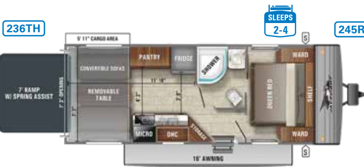
Ext. Lgth: 28' 4" Weight: 4,890 lbs. Hitch: 830 lbs.
