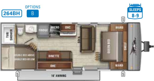
Ext. Lgth: 29' 5" Weight: 4,690 lbs. Hitch: 475 lbs.
