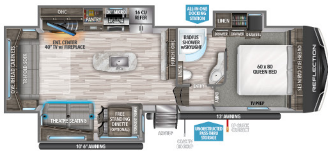
303RLS UVW 1 9,854 HITCH 1 1,865 LENGTH 2 32' 9" HEIGHT 3 12' 3" CAPACITY 74 87 47
