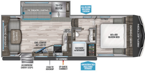
260RD UVW 1 7,534 HITCH 1 1,269 LENGTH 2 29' 9" HEIGHT 3 12' 0" CAPACITY 56 71 39
