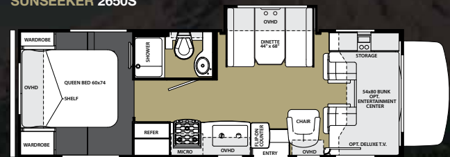
SUNSEEKER 2650S
