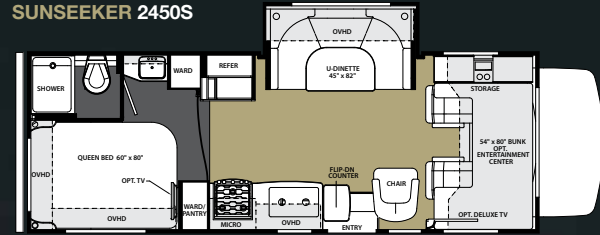
SUNSEEKER 2450S
