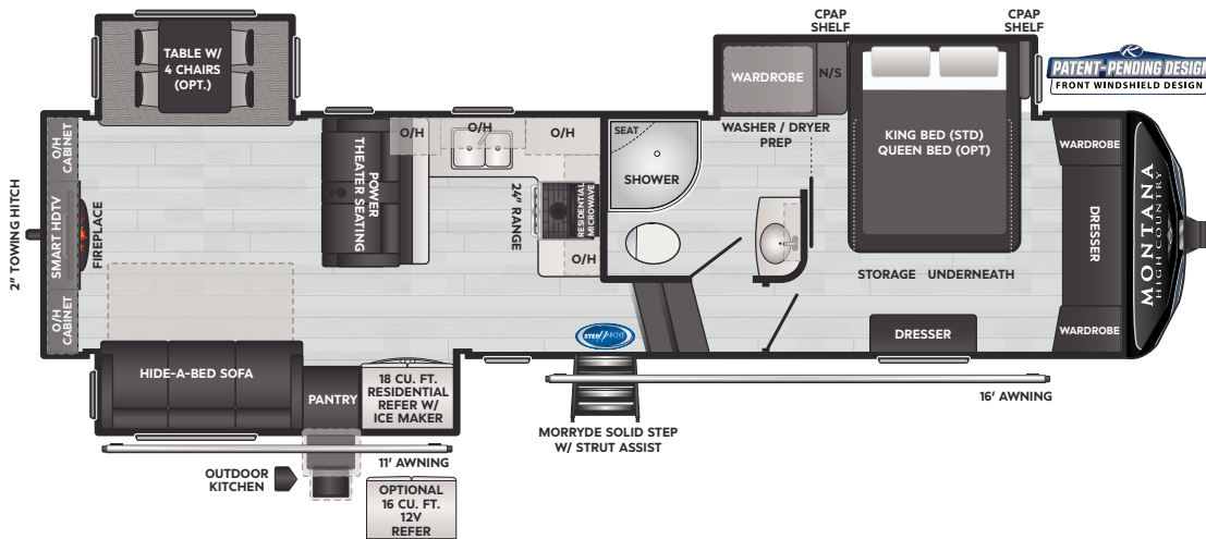
311RD | WEIGHT 11833 | LENGTH 35' 0"
