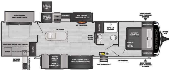
340BH | Bunkhouse, three slides, outside kitchen WEIGHT 8752 LENGTH 38' 6"
