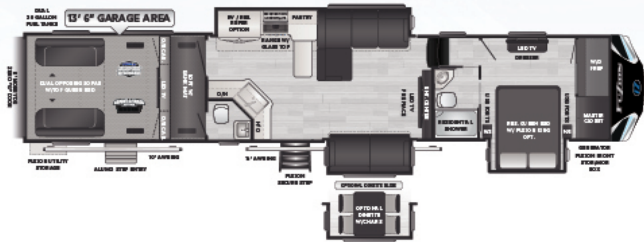
429 L-shaped sofa, 1 1/2 bath, triple-axle, 13' 6" garage WEIGHT 15570 LENGTH 44' 11"
