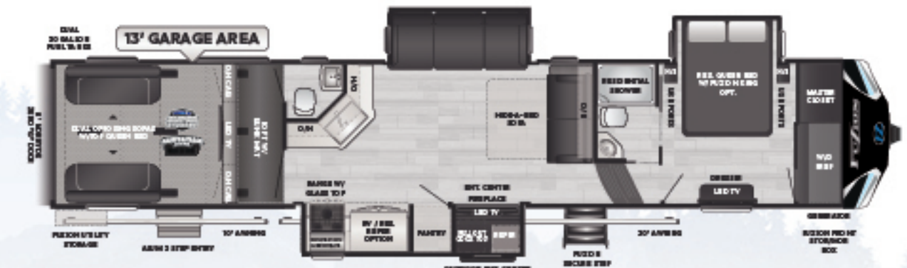
428 Cross conversational seating, 1 1/2 bath, outdoor kitchen, 13' garage WEIGHT 15932 LENGTH 44' 11"
