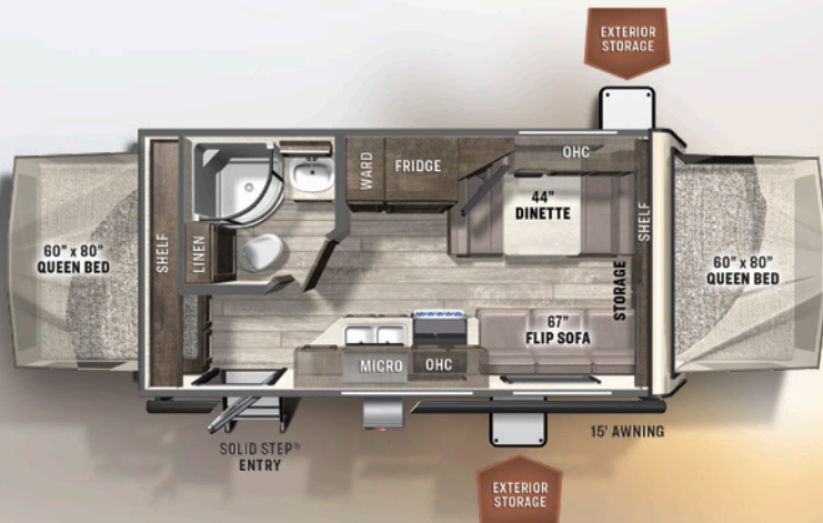
19 EXPANDABLE UUV: 4137 HITCH: 448 AXLE: 3651 LENGTH: 21'2" OPEN LENGTH: 25'7" ROO CCC: 1591 WIDTH: 8' HEIGHT: 10'6" FRESH: 54 gal GRAY: 30gal BLACK: 30gal
