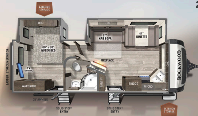
2608BS FRONT KITCHEN UVW: 6836 HITCH: 946 AXLE: 5831 CCC: 1910 LENGTH: 29' 8" ULTRA LITE WIDTH: 8' HEIGHT: 11' 2" FRESH: 54 gal GRAY: 90 gal BLACK: 45 gal
