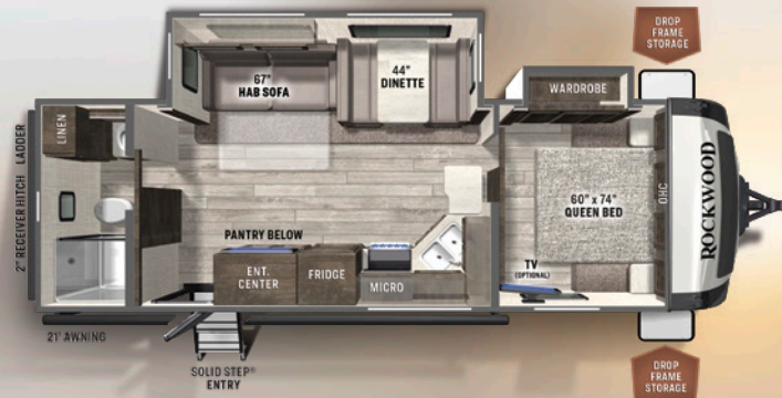
2606WS REAR LIVING UVW: 6158 HITCH: 908 AXLE: 5191 CCC: 2550 LENGTH: 29' 9" ULTRA LITE WIDTH: 8' HEIGHT: 11' 2" FRESH: 54 gal GRAY: 90 gal BLACK: 45 gal
