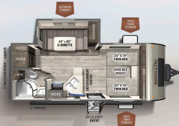
2204S TWIN BED UVW: 4795 HITCH: 640 AXLE: 4096 CCC: 2005 LENGTH: 23' 11" MINI LITE WIDTH: 8' HEIGHT: 10' 11" FRESH: 54 gal GRAY: 30 gal BLACK: 30 gal
