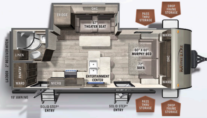
2514S MURPHY BED MINI LITE U/VW: 5879 HITCH: 585 AXLE: 5235 CCC: 1706 LENGTH: 25' 10" WIDTH: 8' HEIGHT: 10' 11" FRESH: 54 gal GRAY: 30 gal BLACK: 30 gal
