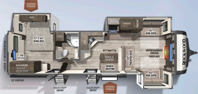
8324SB FRONT LIVING SIGNATURE U/VW: 9254 HITCH: 1115 AXLE: 8080 CCC: 1861 LENGTH: 36' 8" WIDTH: 8' HEIGHT: 11' 7" FRESH: 54 gal GRAY: 120 gal BLACK: 50 gal
