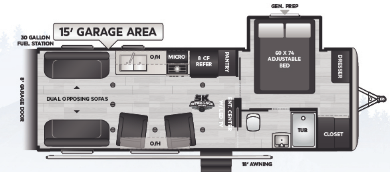
25V Lightweight, one slide, 15' garage WEIGHT 6965 LENGTH 28' 10"
