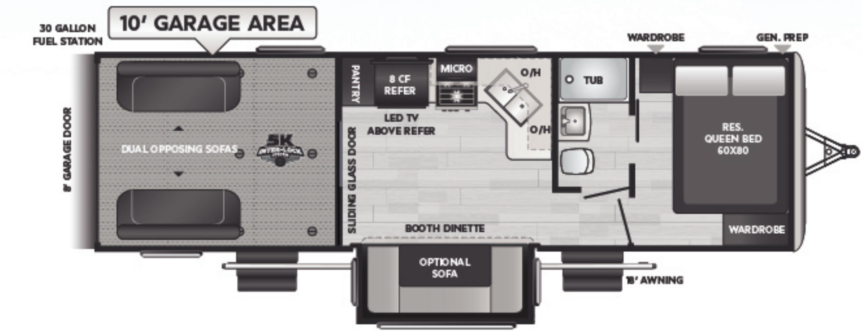
28V Lightweight, one slide, 10' garage WEIGHT 7440 LENGTH 32' 8"
