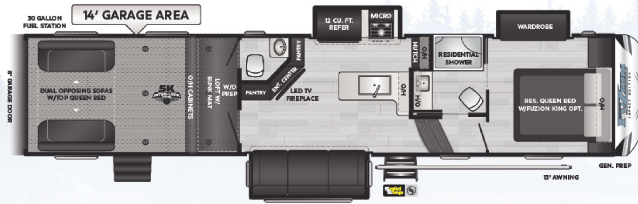
367 Tandem-axle, 1 1/2 baths, 12 cu.ft. refer, 14' garage WEIGHT 13010 LENGTH 40' 2"
