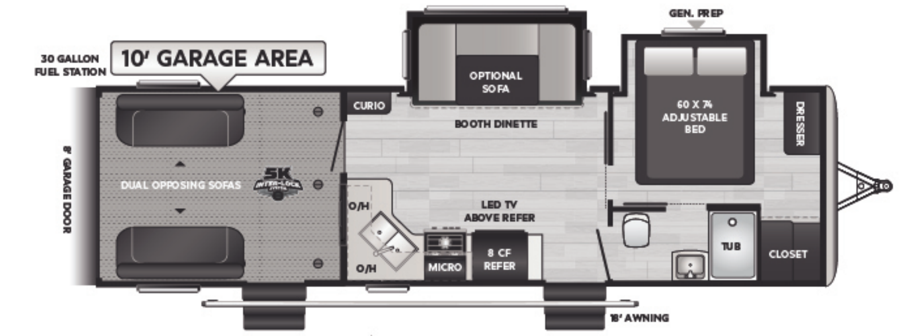
29V Lightweight, two slides, 10' garage WEIGHT 8013 LENGTH 33' 10"
