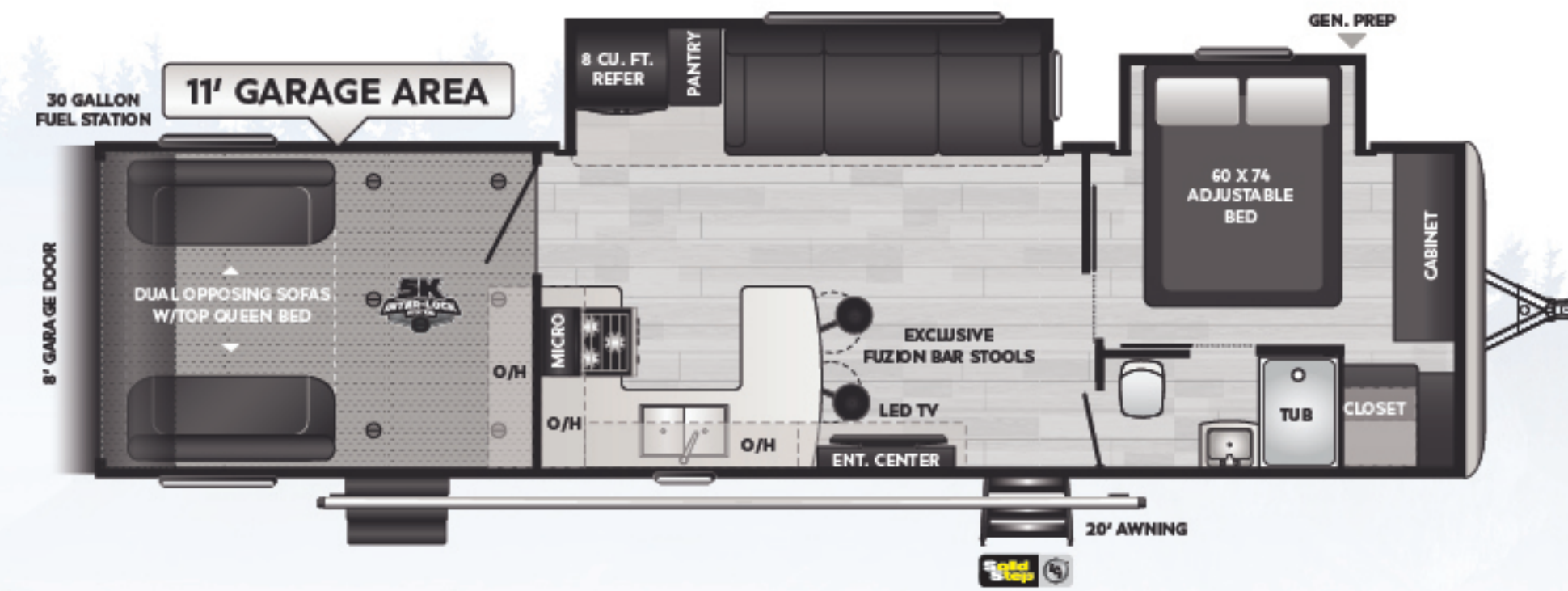
317 U-shaped kitchen, swing out stools, two slides, 11' garage WEIGHT 9700 LENGTH 37' 6"
