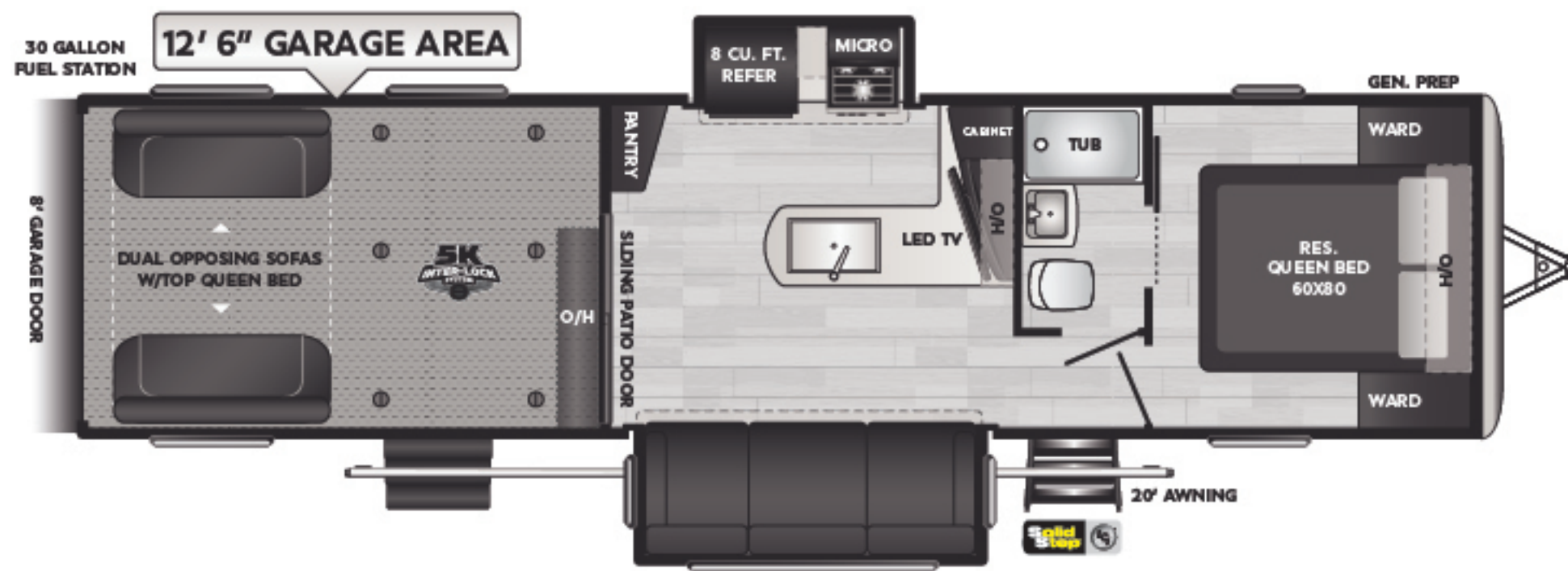
330 Angled entertainment center, two slides, 12' 6" garage WEIGHT 9768 LENGTH 37' 6"
