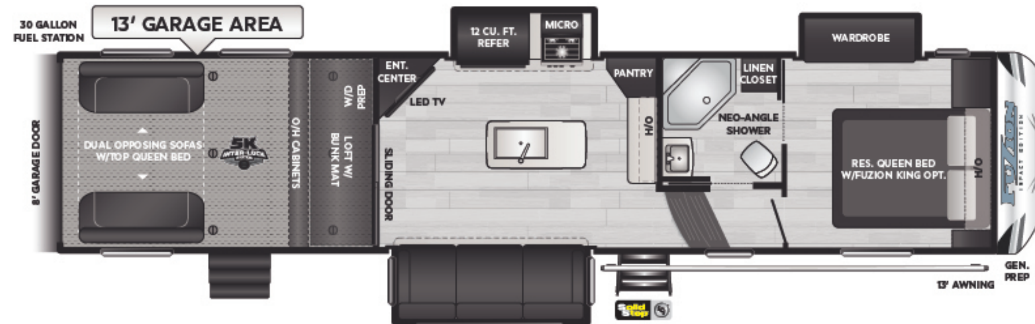
343 Tandem-axle, kitchen island, three slides, 13' garage WEIGHT 12635 LENGTH 39' 0"
