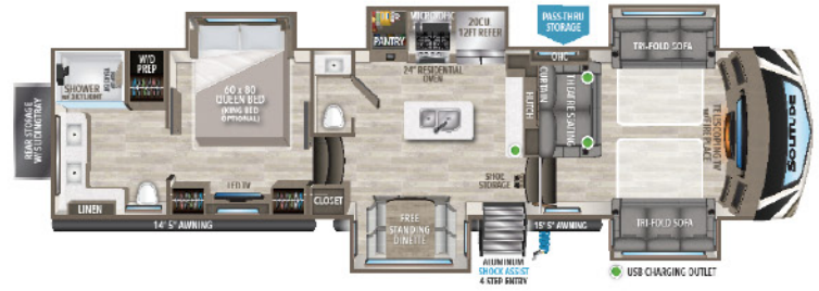
380FL UVW 1 14,866 HITCH 1 3,052 GVWR 16,800 LENGTH 1 41' 5" HEIGHT 13' 5" CAPACITY 81 106 106
