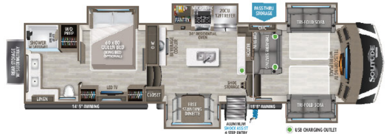
382WB UVW 1 14,866 HITCH 1 3,052 GVWR 16,800 LENGTH 1 41' 5" HEIGHT 13' 5" CAPACITY 81 106 53
