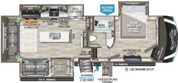
310GK UVW 1 12,100 HITCH 1 2,350 GVWR 15,000 LENGTH 1 34' 11" HEIGHT 13' 5" CAPACITY 81 106 53
