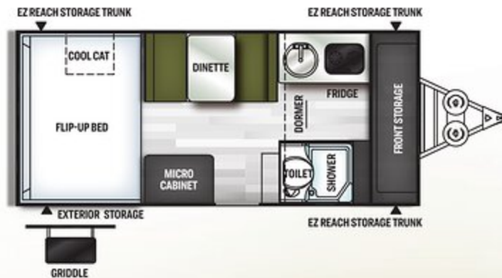
T21DMHW HARD SIDE FLAGSTAFF UVW: 2700 CCC: 653 AXLE: 2309 HITCH: 353 CLOSED HEIGHT: 5'8" CLOSED LENGTH W/ HITCH: 21'2" BOX SIZE: 14' FRESH: 20 GRAY: N/A BLACK: N/A
