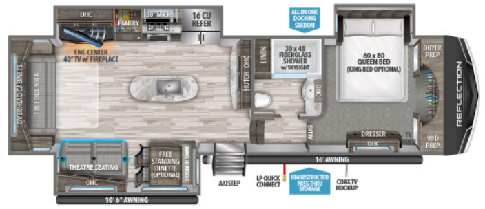
337RLS UVW 1 10,838 HITCH 1 2,185 LENGTH 2 35' 6" HEIGHT 3 12' 6" CAPACITY 74 87 47
