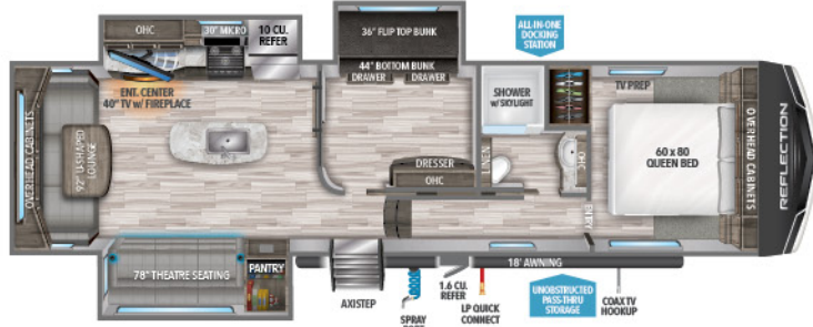
31MB UVW 1 9,906 HITCH 1 1,893 LENGTH 2 36' 2" HEIGHT 3 12' 3" CAPACITY 74 75 43
