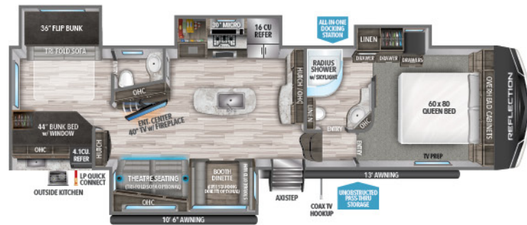
311BHS UVW 1 11,377 HITCH 1 2,316 LENGTH 2 36' 10" HEIGHT 3 12' 3" CAPACITY 74 87 87
