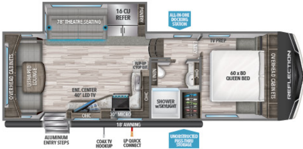
260RD UVW 1 7,534 HITCH 1 1,269 LENGTH 2 29' 9" HEIGHT 3 12' 0" CAPACITY 56 71 39
