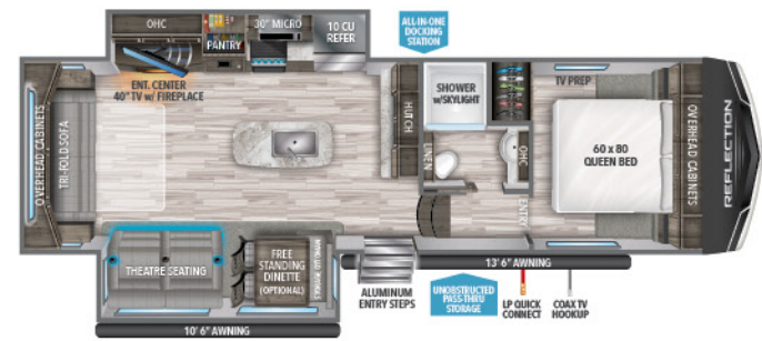
295RL UVW 1 8,995 HITCH 1 1,434 LENGTH 2 32' 9" HEIGHT 3 12' 4" CAPACITY 56 78 39
