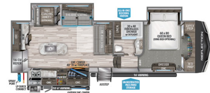
320MKS UVW 1 10,721 HITCH 1 2,076 LENGTH 2 34' 8" HEIGHT 3 12' 6" CAPACITY 74 94 47
