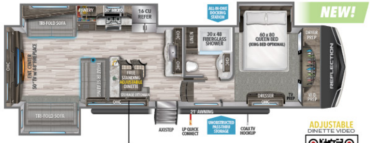
341RDS UVW 1 10,964 HITCH 1 2,072 LENGTH 2 36' 11" HEIGHT 3 12' 6" CAPACITY 74 87 47
