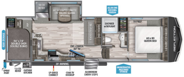
278BH UVW 1 8,345 HITCH 1 1,321 LENGTH 2 32' 11" HEIGHT 3 12' CAPACITY 56 78 39
