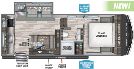
226RK UVW 1 7,204 HITCH 1 1,190 LENGTH 2 26' 11" HEIGHT 3 12' 0" CAPACITY 56 71 39
