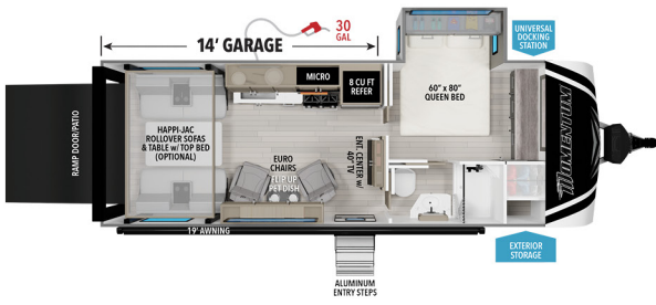
21G 14' GARAGE UVW 1 EMPTY HITCH 1 GVWR LENGTH 1 HEIGHT CAPACITY 6,400 920 11,000 26' 11" 12' 4" 90 74 39
