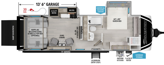
25G 13' 6" GARAGE UVW 1 EMPTY HITCH 1 GVWR LENGTH 1 HEIGHT CAPACITY 7,900 1,150 13,000 30' 11" 12' 4" 90 78 39
