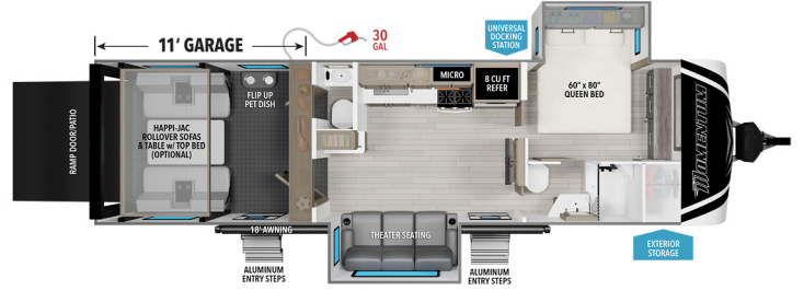
29G 11' GARAGE UVW 1 EMPTY HITCH 1 GVWR LENGTH 1 HEIGHT CAPACITY 9,278 1,592 13,000 33' 11" 12' 4" 90 37 39 37* * 1/2 BATH DOUBLES AS BLACK/GREY
