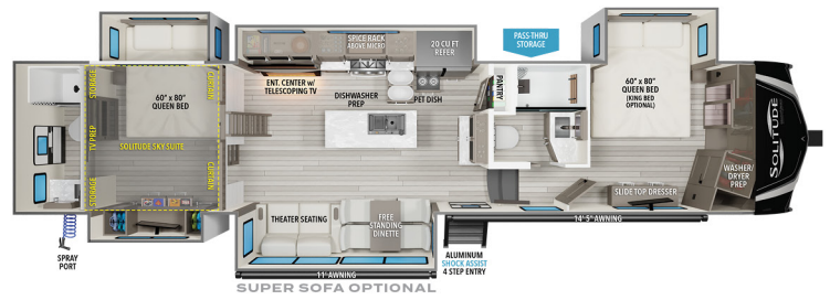
391DL U W # HITCH# GVWR LENGTH# HEIGHT CAPACITY 15,300 3,050 18,000 42' 5" 13' 5" 81 106 106
