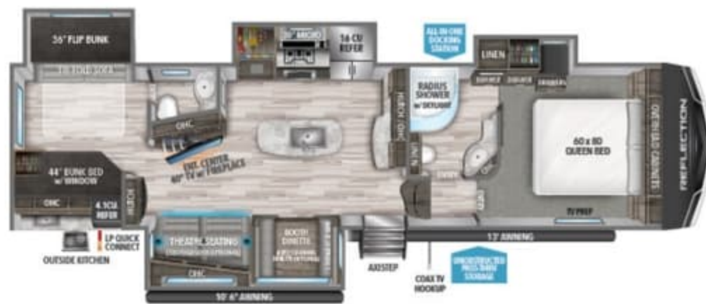
311BHS UVW 1 11,377 HITCH 1 2,316 LENGTH 2 36' 10" HEIGHT 3 12' 3" CAPACITY 74 87 87
