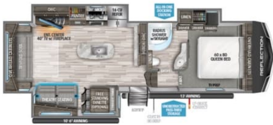
303RLS UVW 1 9,854 HITCH 1 1,865 LENGTH 2 32' 9" HEIGHT 3 12' 3" CAPACITY 74 87 47
