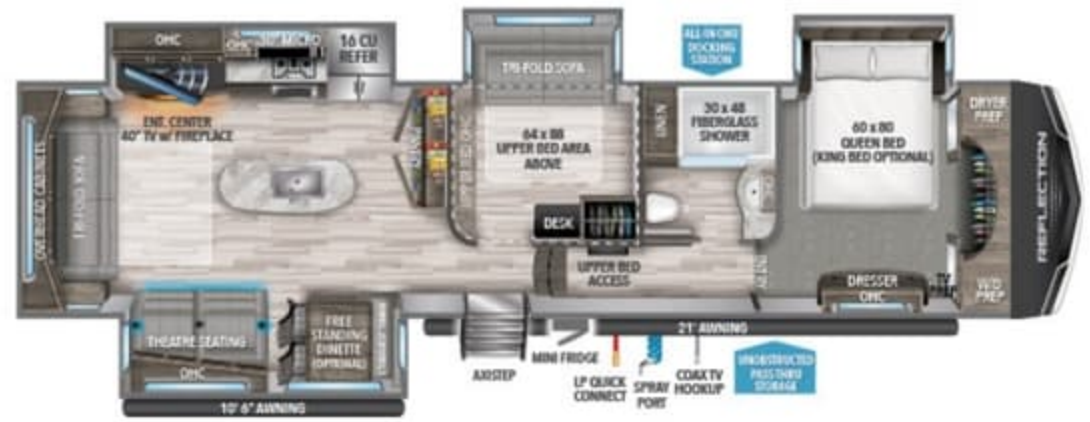
367BHS UVW 1 12,552 HITCH 1 2,461 LENGTH 2 41' 0" HEIGHT 3 12' 8" CAPACITY 74 94 47
