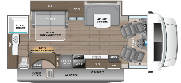
26M Theater Sofa Option ILO Dinette
