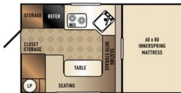
1/2 TON TRUCK W/ 6' 6" OR 8' BED
