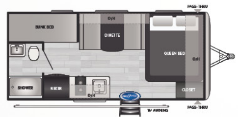
1800BH | WEIGHT 3396 | LENGTH 21' 5"
