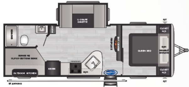
240BHWE WEIGHT 5915 LENGTH 28' 11" • #1 SELLING FLOORPLAN
