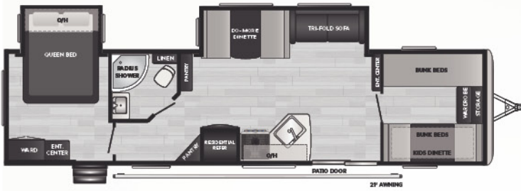
38BH | WEIGHT 8994 | LENGTH 38' 11"
