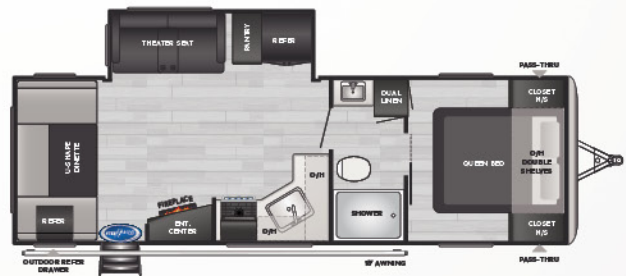
256RDWE WEIGHT TBD LENGTH TBD • REAR DINETTE W/ PANORAMIC VIEW
