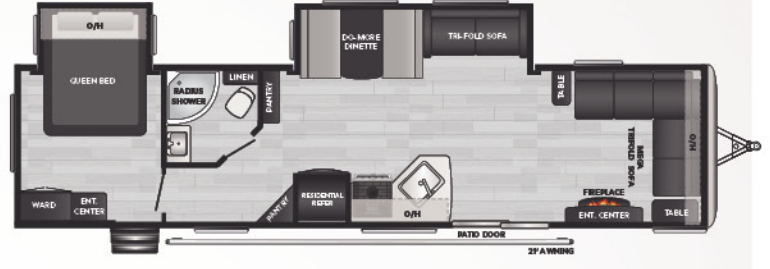
38FL | WEIGHT 8725 | LENGTH 38' 11"
