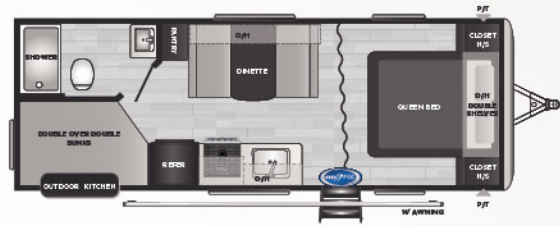
220BHWE WEIGHT 4880 LENGTH 26' 11" • DOUBLE BUNKS, OUTDOOR KITCHEN
