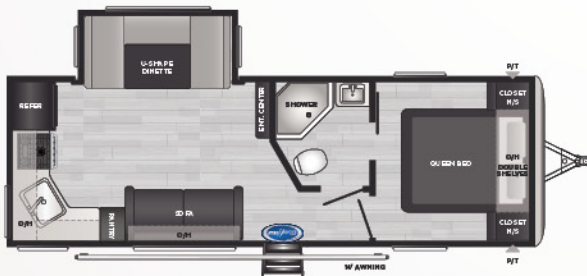
242RKWE WEIGHT 5827 LENGTH 28' 8" • SMALL SLIDE, REAR KITCHEN, DUAL ENTRY BATH
