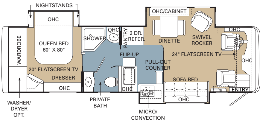
34' Bayview III Floorplan
