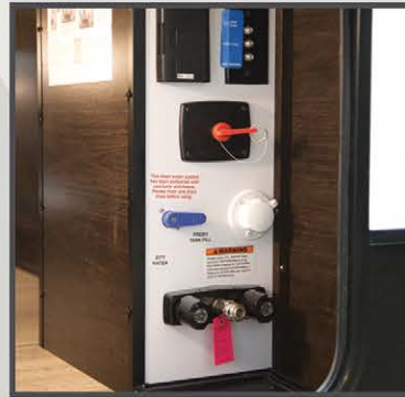
UNIVERSAL DOCKING STATION All-in-one location for utilities and hookups.
