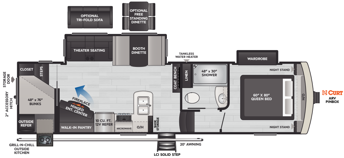
288SLBH | WEIGHT 8857 | LENGTH 32' 8"
