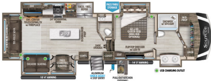
373FB 373FB-R U 1 VW 1 HITCH 1 GVWR LENGTH 1 HEIGHT CAPACITY 13,950 2,800 16,800 41' 4" 13' 5" 93 100 100
