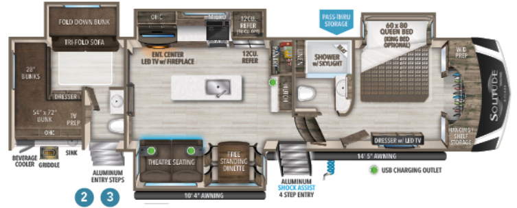
3740BH U/VW 1 HITCH 1 GVWR LENGTH 1 HEIGHT CAPACITY 3740BH-R 13,884 2,900 16,800 40' 4" 13' 5" 91 106 106
