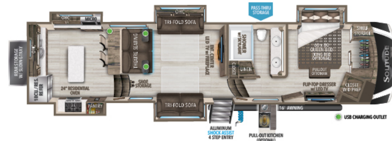
390RK U/VW 1 HITCH 1 GVWR LENGTH 1 HEIGHT CAPACITY 390RK-R 14,562 2,794 16,800 41' 5" 13' 5" 93 106 53
